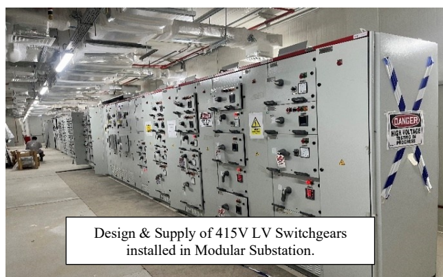
LV Panels
