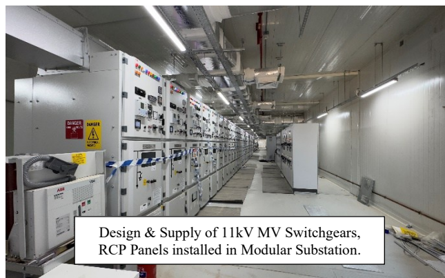
MV Panels
